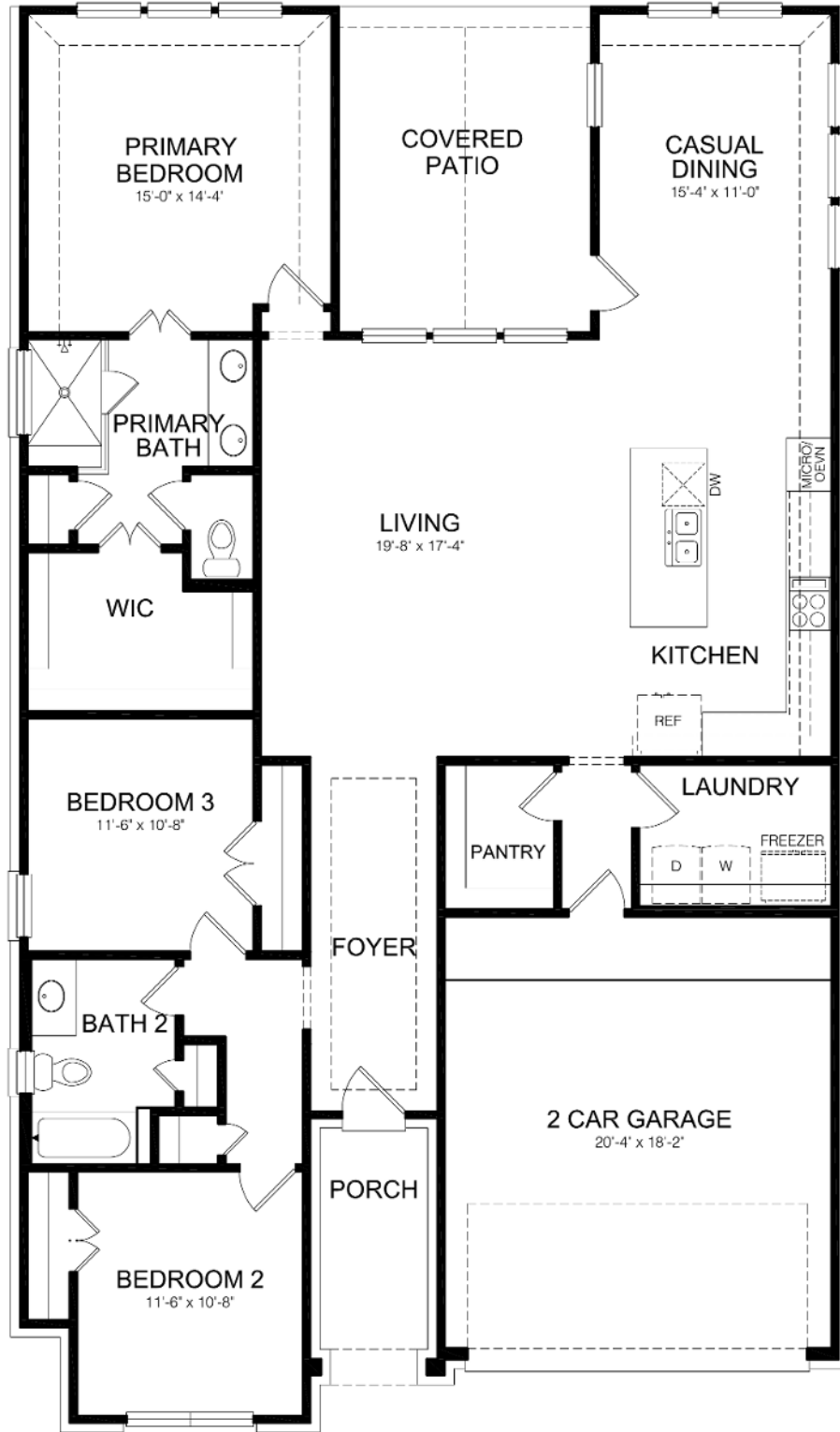
MAIN FLOOR PLAN ELEVATION J
