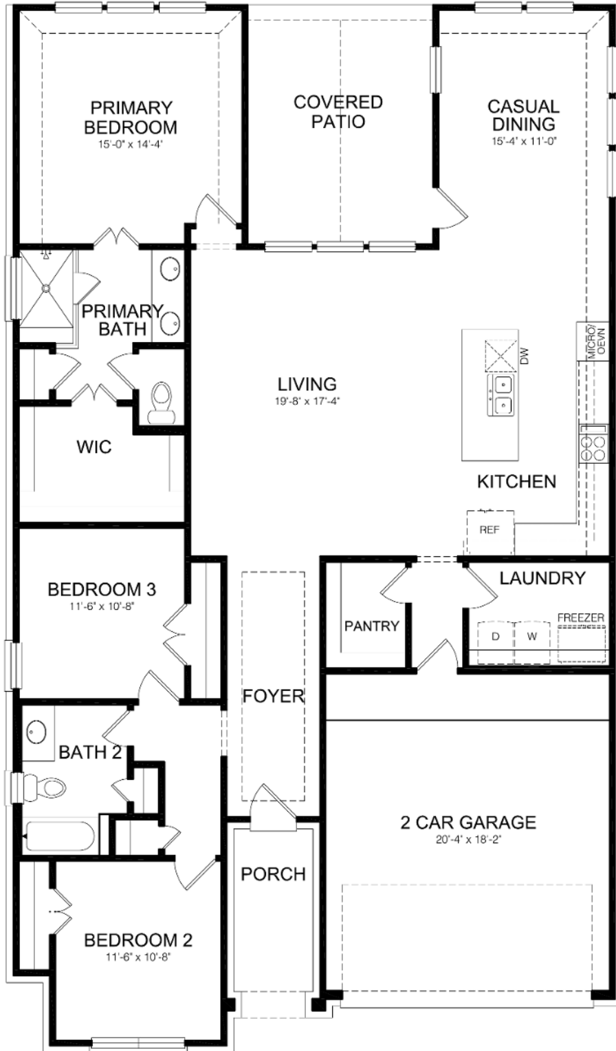
MAIN FLOOR PLAN ELEVATION D
