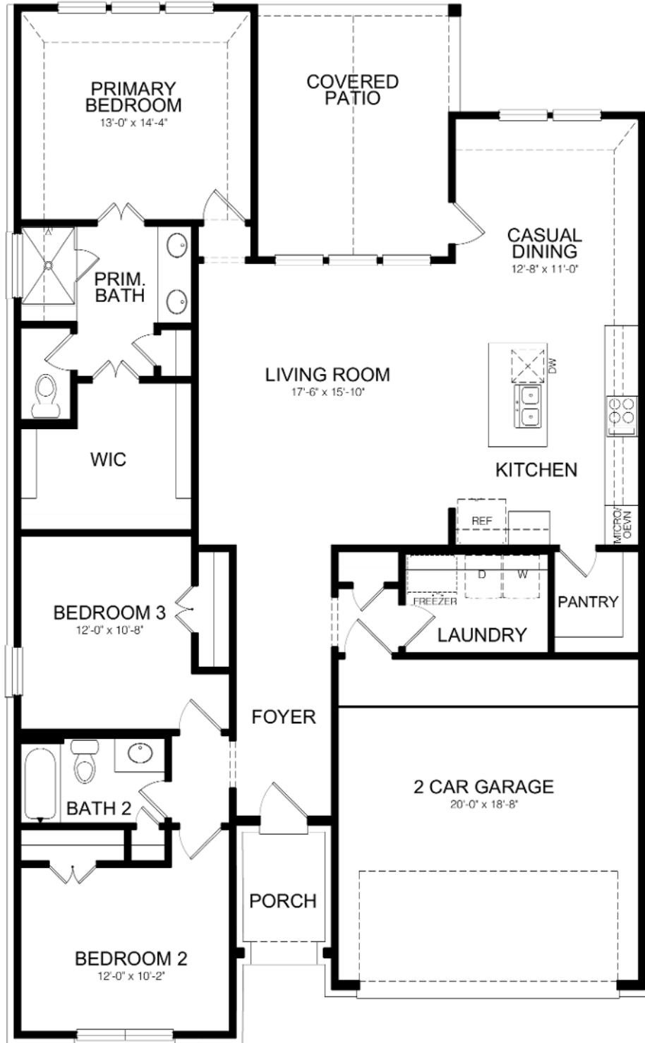
MAIN FLOOR PLAN ELEVATION G
